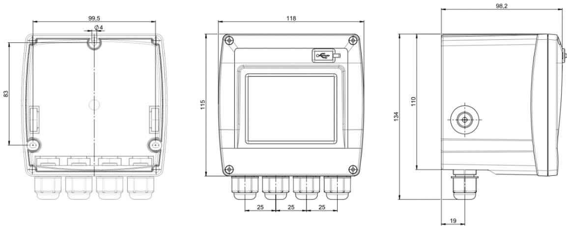
Figure : Housing for wall mounting
