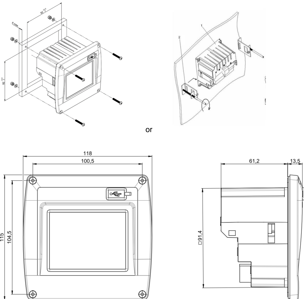
Figure : Housing for panel mounting
