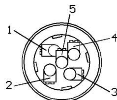
M12 Connector plug
